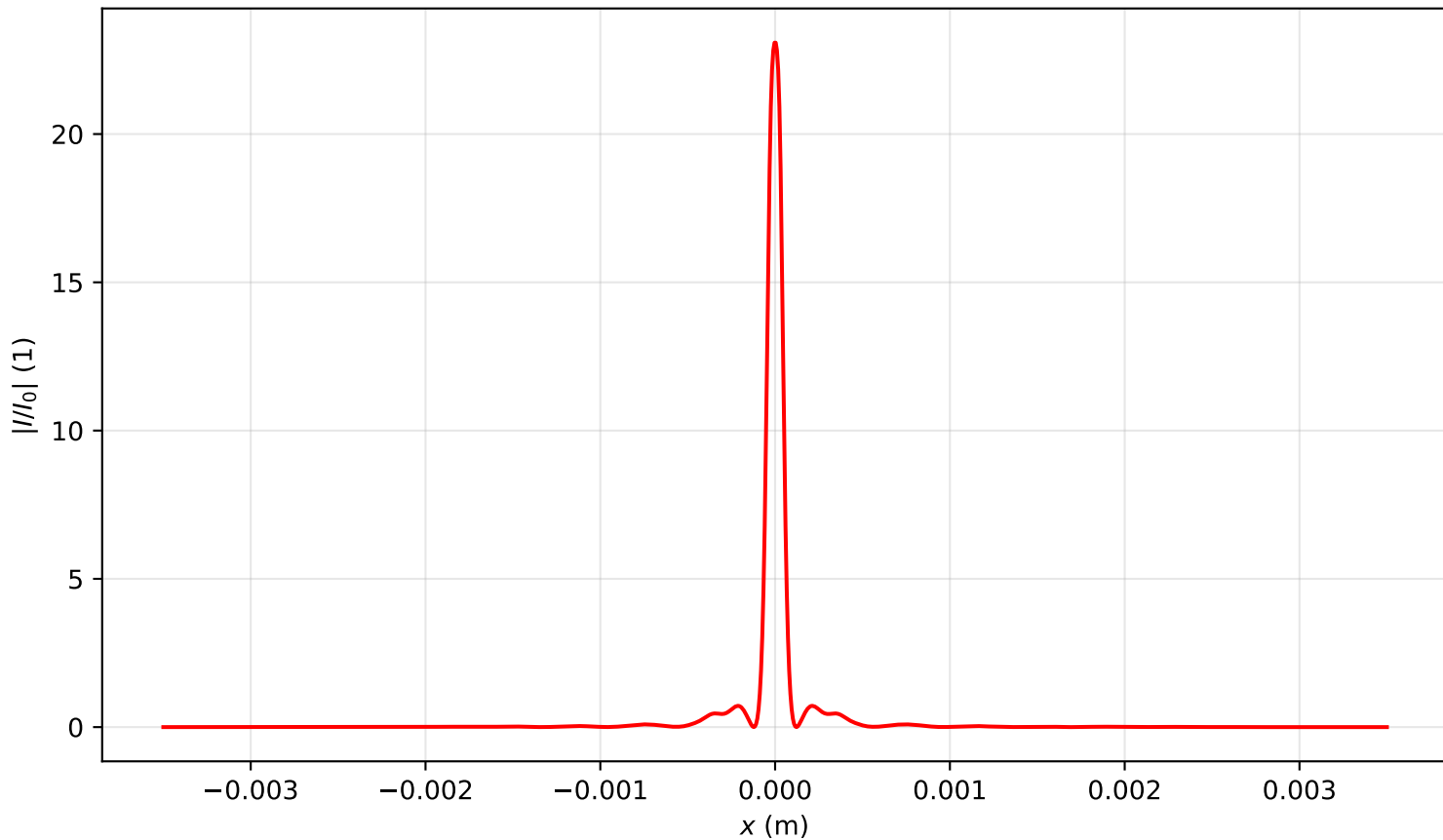
Intensity profile I(x, y = 0, z = 0.318)/I_0 , P_{in}=3.0P_{cr} , artificial time
